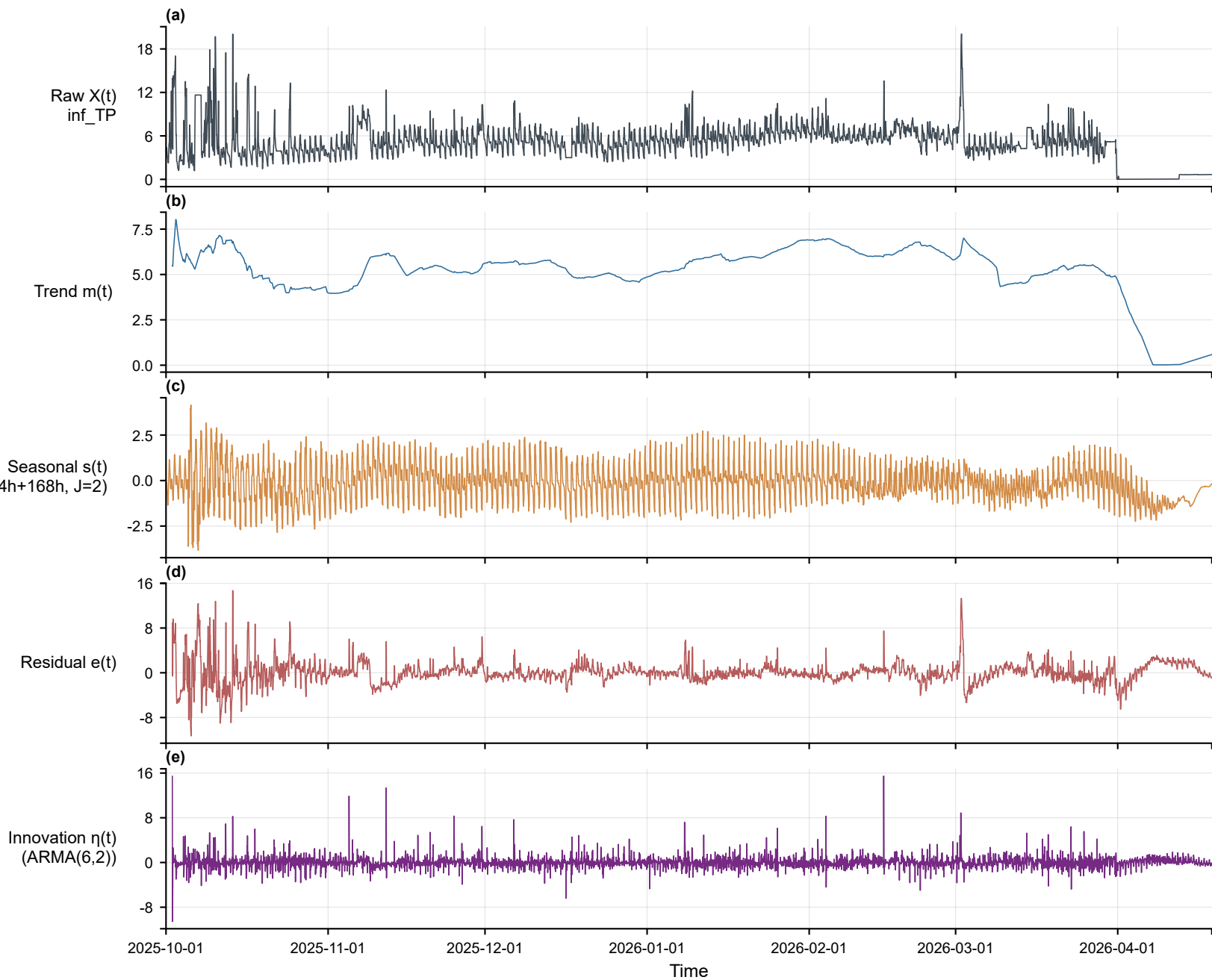
Multi-scale decomposition — inf_TP (influent, hour) [2025-10-01~2026-04-19]
